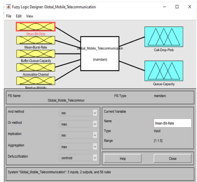
Fig 5: MATLAB input diagram
