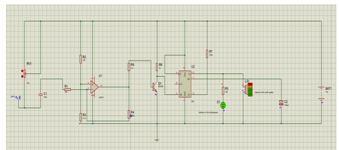
Fig -2: After simulation of circuit
