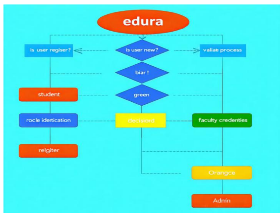
Fig. 8.1 Flowchart
