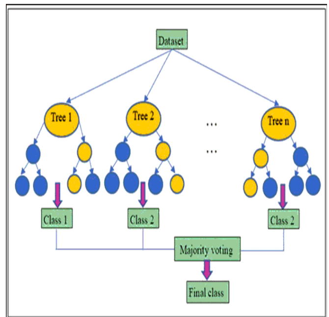
Fig. -8: Random Forest
