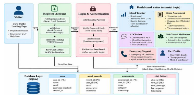
Fig. 1. System Architecture of the Proposed Digital Mental Health Support System
