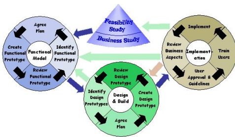
Fig 1.5: DSDM Process
