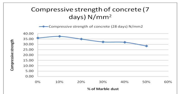
Chart-2: Compressive strength of concrete mix at 7 days
