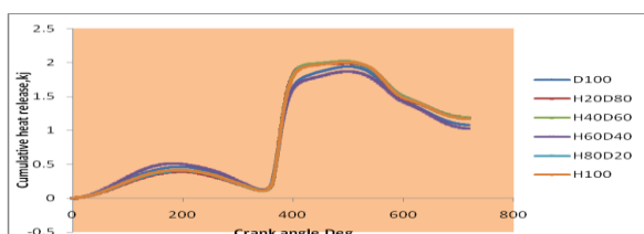
Fig.12 Variation of crank angle with cumulative heat release rate
