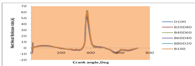
Fig.11 Variation of crank angle with net heat release rate
