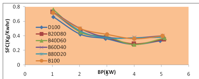
Fig.3variation of specific fuel consumption with brake power
