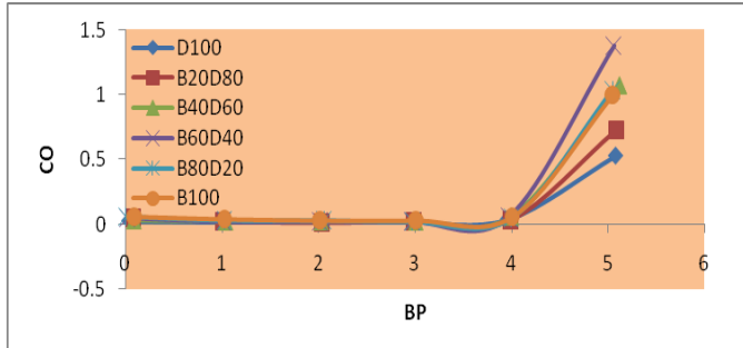
Fig.6 Variation of carbon monoxide emission with brake power
