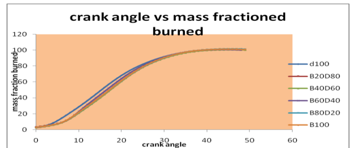
Fig.13 Variation of crank angle with cumulative heat release rate
