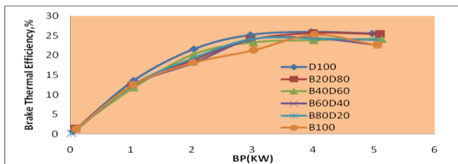
Fig.2 variation of brake thermal efficiency with brake power
