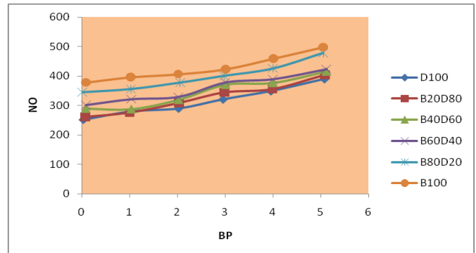
Fig. 8 The variation of the nitrogen oxide with brake power for diesel and corn blends.
