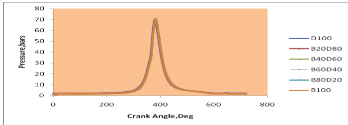
Fig.10 Variation of crank angle with with pressure
