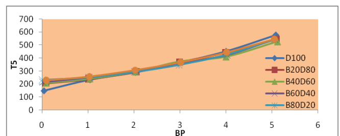
Fig5.Variation of exhaust gas temperature with BP
