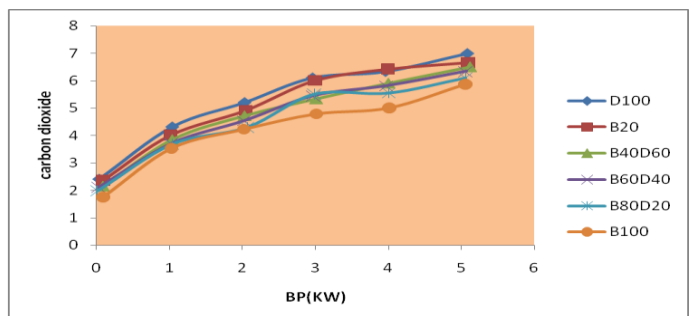
Fig.10 Variation of carbon dioxide emission with brake power
