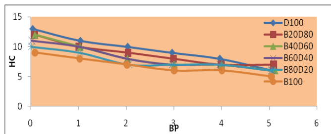
Fig. 7 Variation of hydrocarbon emission with brake power
