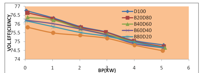
Fig.4 Variation of volumetric Efficiency with brake power
