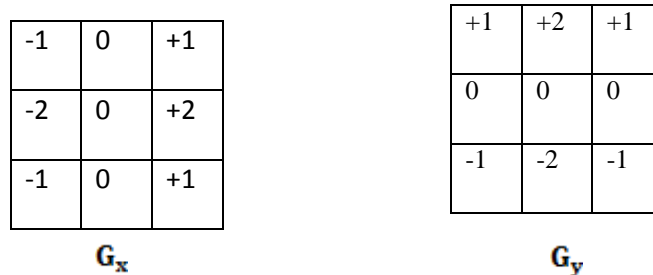
Fig-1: Sobel convolution kernels
