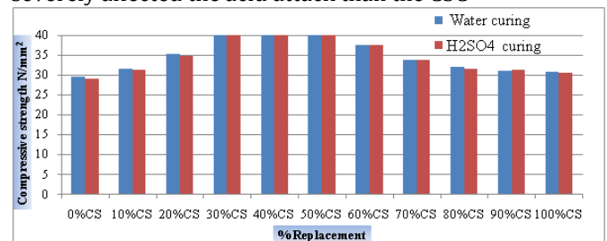
Chart-3: Compressive Strength(H2SO4) Vs. % Replacement
