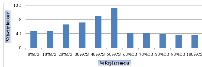
Chart-4: Pulse Velocity Vs. % Replacement
