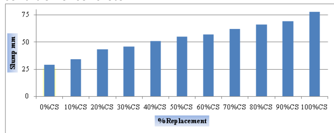
Chart-2: Slump Vs. % Replacement
