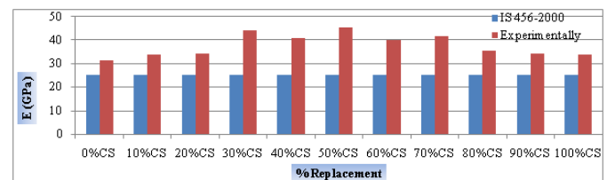
Chart-5: Modulus Of Elasticity ( E ) Vs. % Replacement
