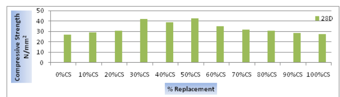
Chart-1: Compressive Strength (MPa) Vs. % Replacement
