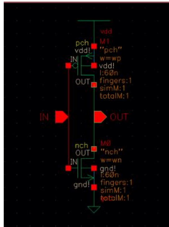
Fig:3 Schematic diagram of CMOS inverter
