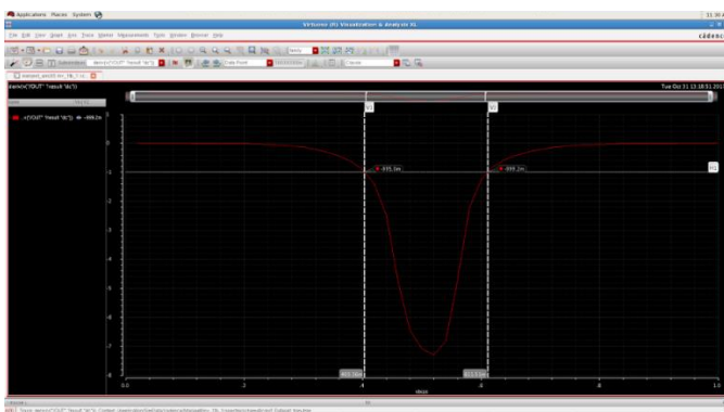
Fig 7: VTC derivative curve of CMOS inverter.
