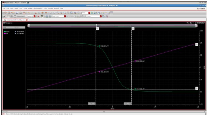
Fig 6 : VTC of the CMOS inverter.
