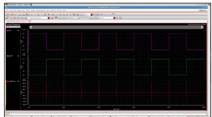
Fig 5: Transient behavior of CMOS inverter (i) V_{IN} (ii) V_{OUT} (iii) I_C
