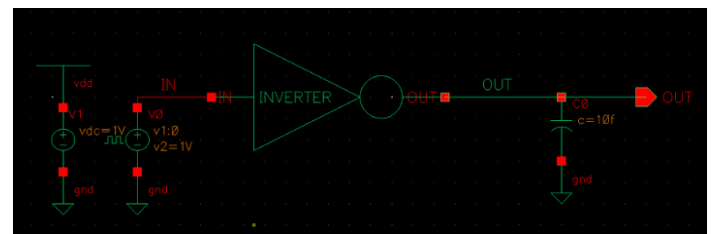
Fig 4: Transient analysis of CMOS inverter with C_L as a load
