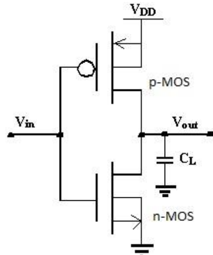
Fig 1: Structure of CMOS inverter
