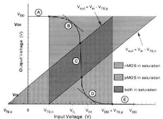
Fig 2: Operating region of n-MOS and p-MOS transistor [1]
