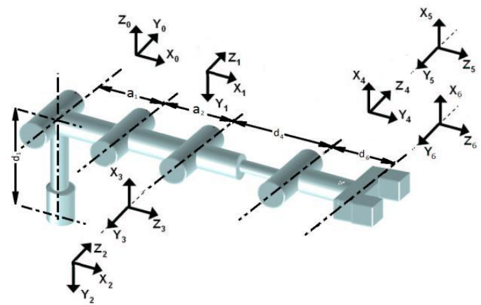
Fig 4: Coordinate frame for the 5-DOF Redundant manipulator
