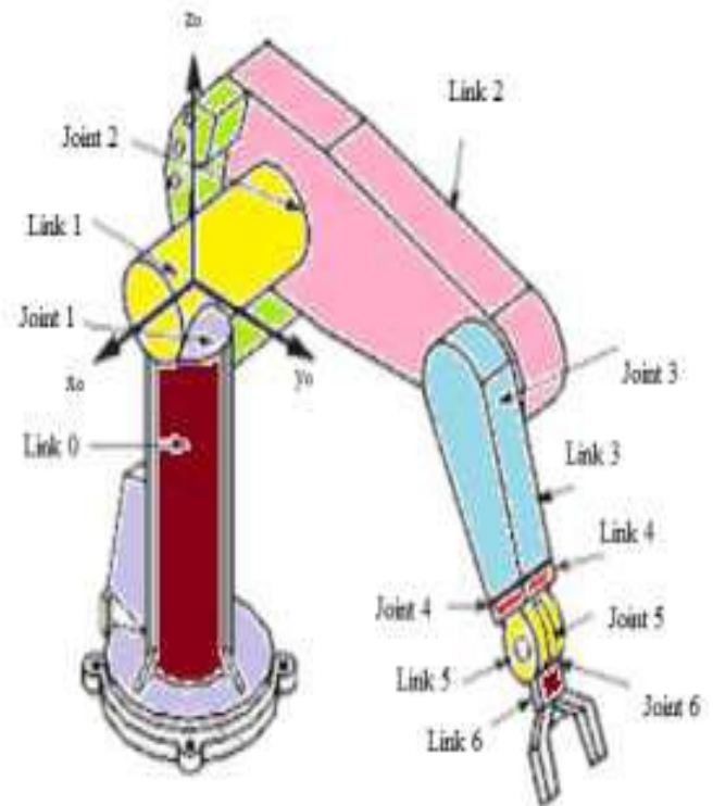
Fig 5: Puma 560 6DOF robot with frame assignment
