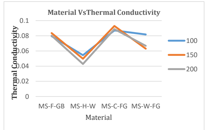
Graph 7.3 Materials Vs Thermal conductivity
