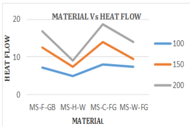
Graph 7.2 Materials Vs Heat Flow Rate
