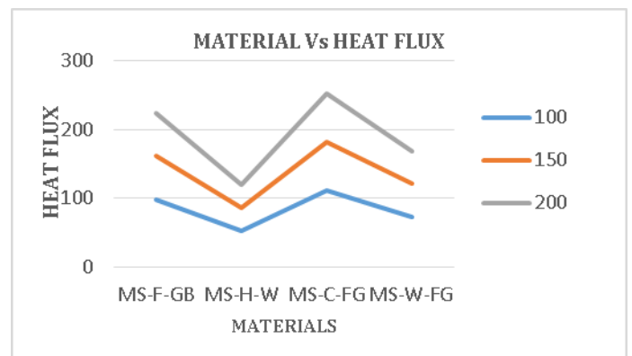
Graph 7.4 Materials Vs Heat Flux
