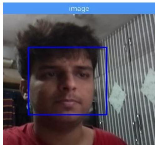
Fig 10. Recording Dataset
