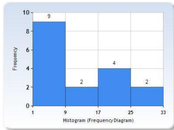
Fig 5. Sample Histogram[7]
