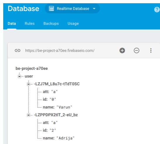
Fig 6. Sample Firebase Database
