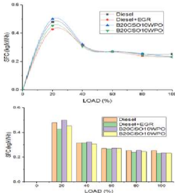
Fig- 5: Variation of SFC
