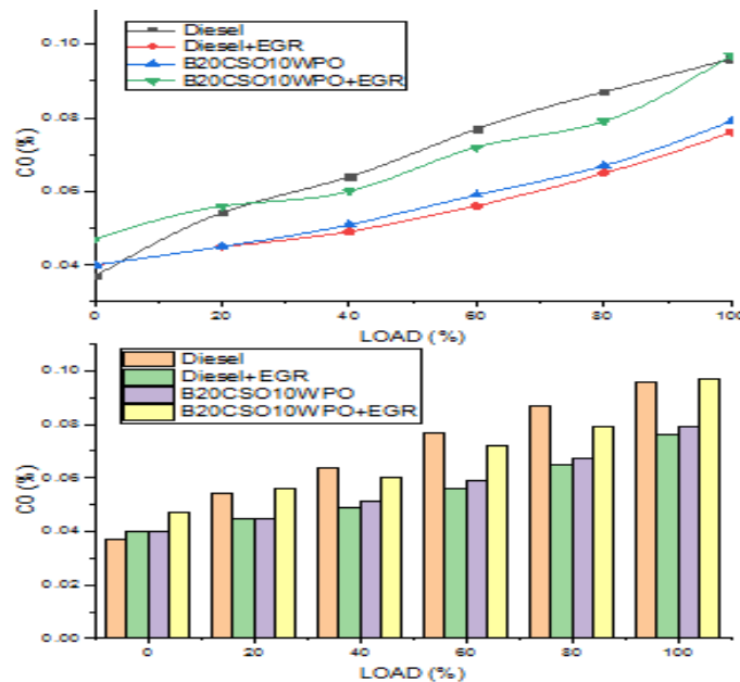
Fig-7: Variations of CO
