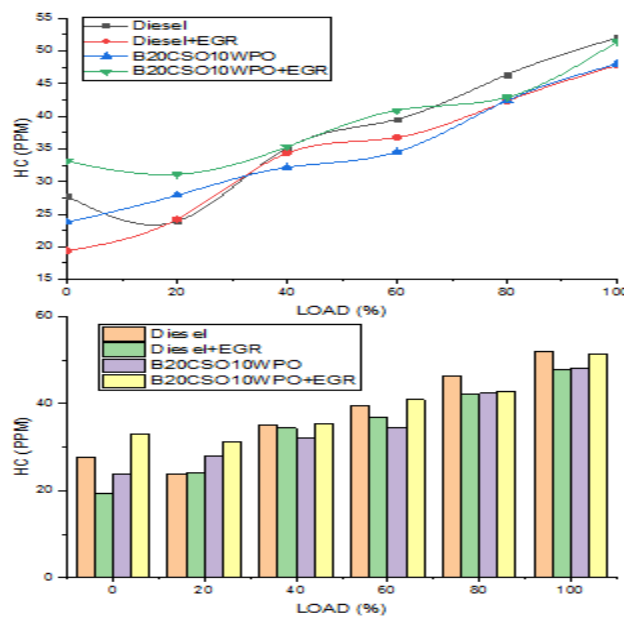
Fig-9: Variation of UBHC
