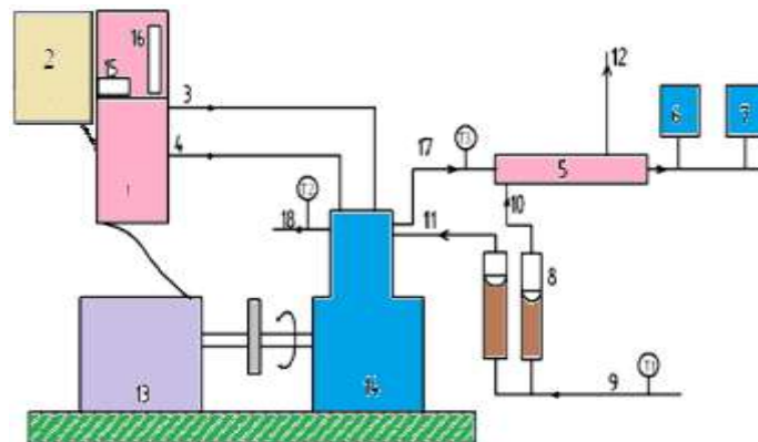
Fig-3: Schematic Diagram of the Experimental Set Up
