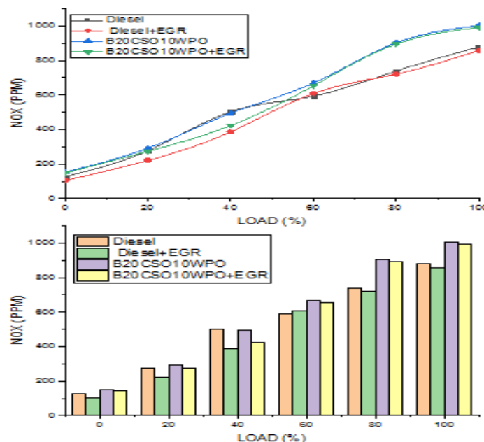
Fig-8: Variation of NOx
