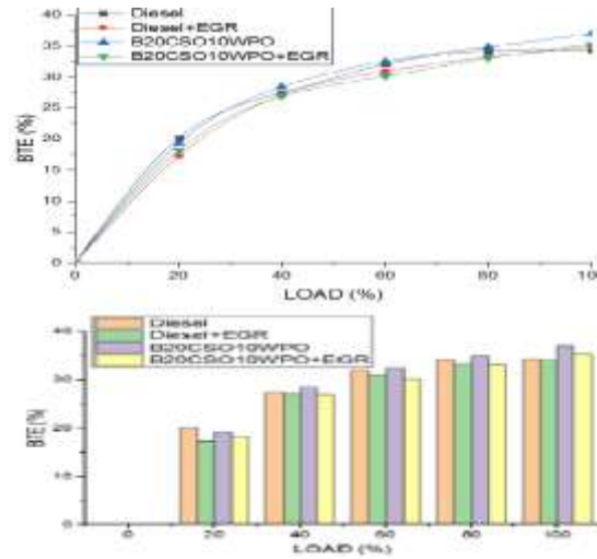
Fig-4: Variations of brake thermal efficiency
