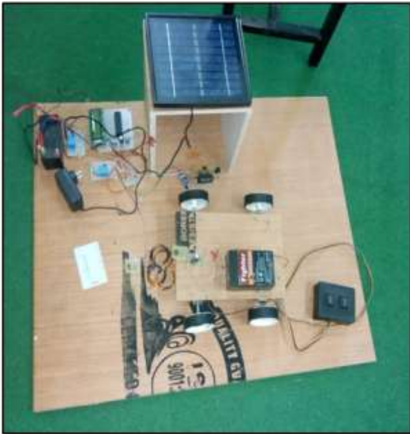
Fig.4: Hardware of Project
