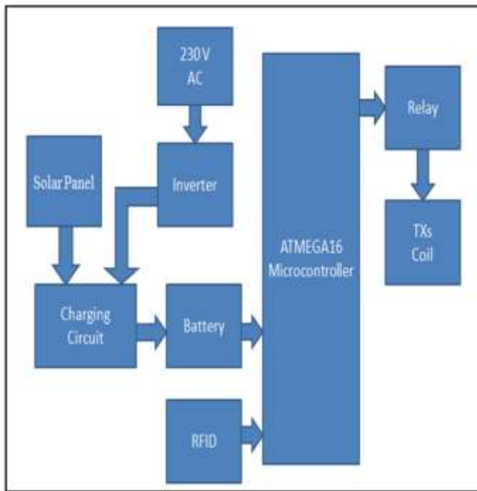
Fig.2: Transmitter Circuit
