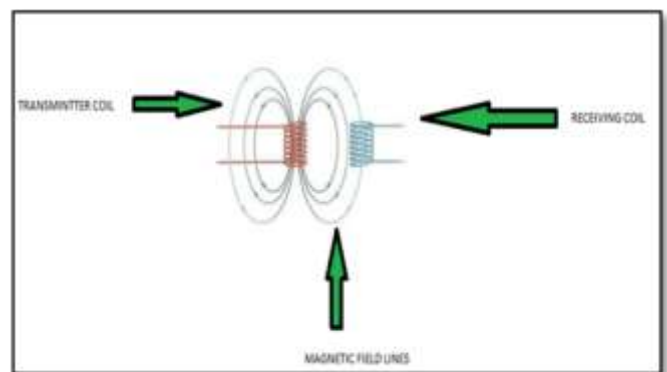
Fig.1: Inductive loosely coupled coil
