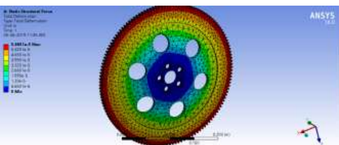
Fig -11: Total Deformation
