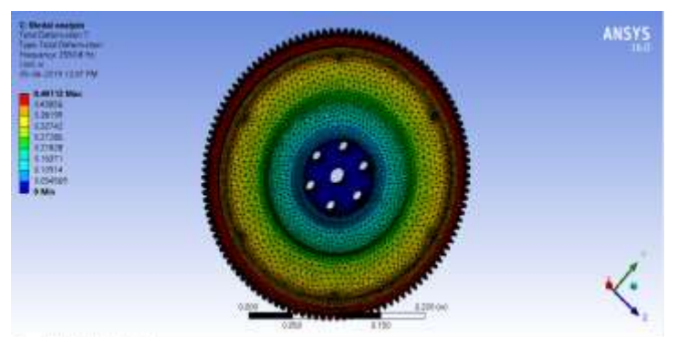
Fig -23: Flywheel iteration 3 – Modal Frequency 6 – Total Deformation
