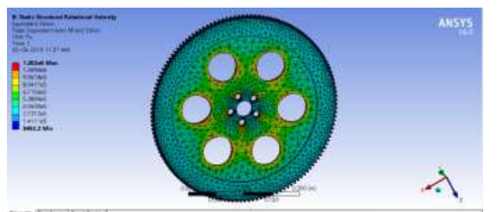
Fig -20: Equivalent Stress (von Mises)
