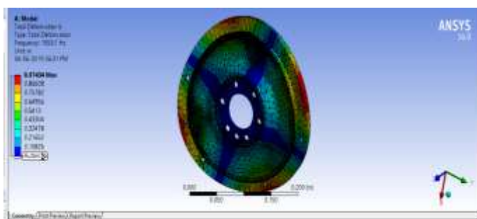
Fig -21: Flywheel iteration 1 – Modal Frequency 6 – Total Deformation
