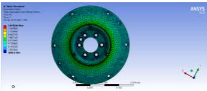
Fig -14: Equivalent Stress (von Mises)
