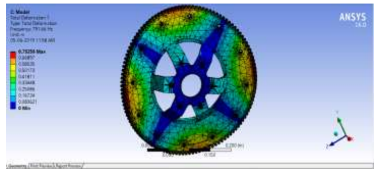
Fig -22: Flywheel iteration 2 – Modal Frequency 6 – Total Deformation
