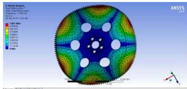
Fig -24: Flywheel iteration 4 – Modal Frequency 6 – Total Deformation
