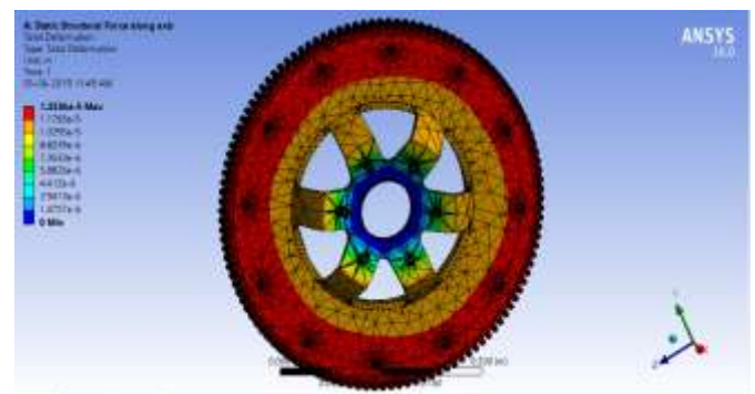
Fig -7: Total Deformation
