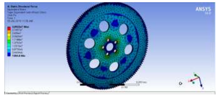
Fig -12: Equivalent Stress (von Misses)
