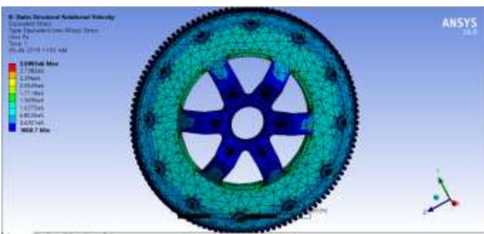
Fig -16: Equivalent Stress (von Mises)
