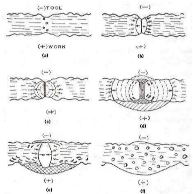
Figure 2.1: Successive stages of discharge
