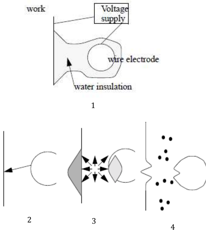
Figure 2.2: The mechanism involved in wire-cut EDM process
