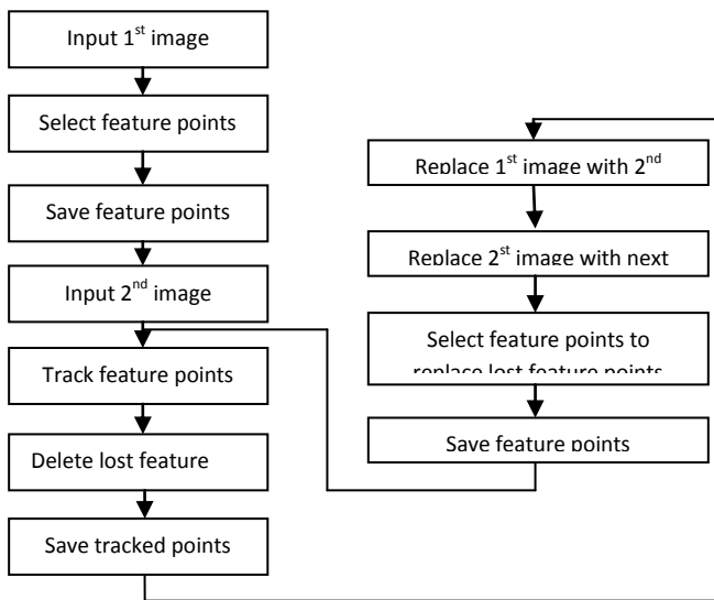
Fig-3: Flowchart KLT
