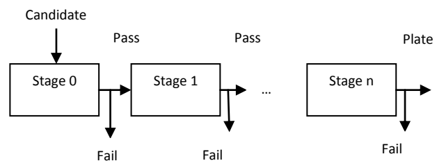
Fig -2: Cascade of Classifiers
