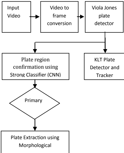
Fig -6: Methodology of Proposed work
