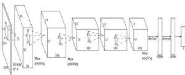
Fig-4: AlexNet
