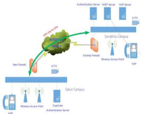
Fig-1: Campus Network VPN
