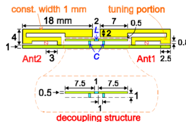
Figure 1 (b): Side view of the antenna part and feeding part
