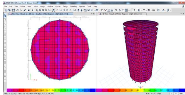
Fig -5: Stresses on building due to dynamic analysis
