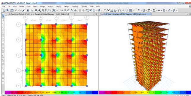
Fig -3: Stresses on building due to dynamic analysis
