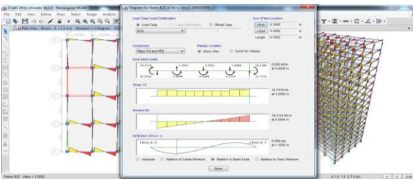
Fig -2: Moment on beams
