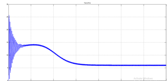
Figure 10 Electro-mechanical torque Vs. Time
