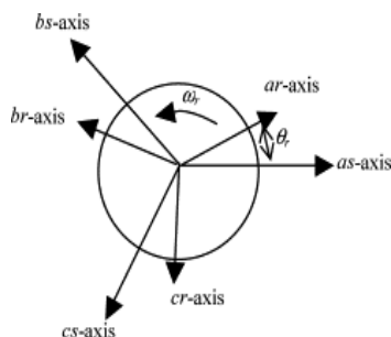
Figure 1 Induction machine winding displacement
