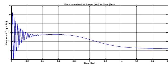
Figure 5. Electro-mechanical torque Vs. Time
