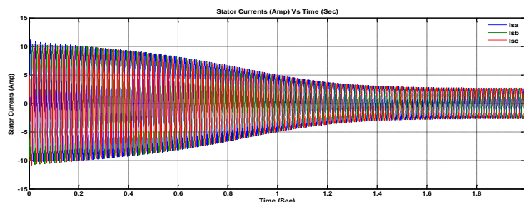
Figure 3. Stator currents Vs. time
