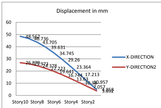
Fig. 4.2 Displacement X and Y Direction of the structure in zone 4
