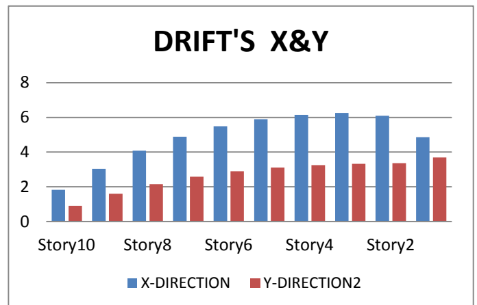
FIG. 4.3 COMPARISON OF DRIFTS X AND Y IN ZONE 4
