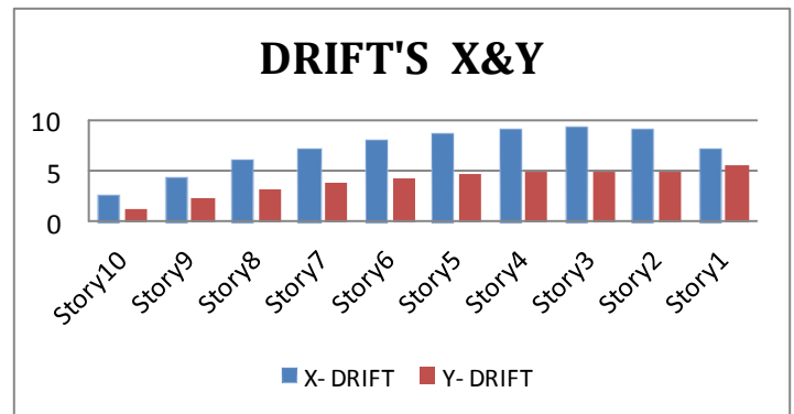
Fig. 4.2 Comparison Of Drifts X And Y In Zone 5
