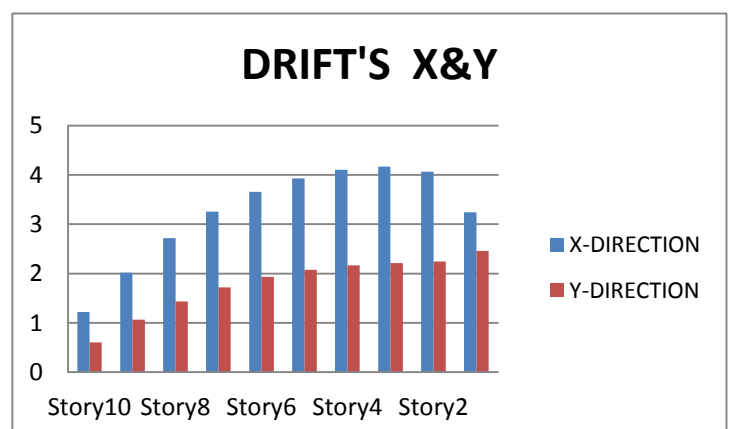
FIG. 4.6 COMPARISON OF DRIFTS X AND Y IN ZONE 3
