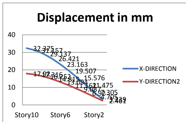
Fig. 4.5 Displacement X and Y Direction of the structure in zone 3
