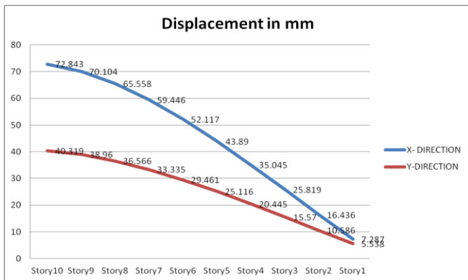
Fig. 4.1 Displacement X and Y Direction of the structure in zone 5
