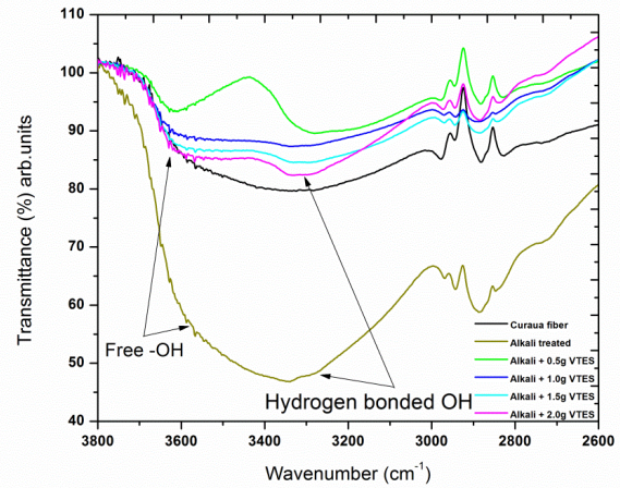
Figure 2. FTIR spectra showing OH groups of untreated, NaOH treated, and NaOH and silane treated curaua fiber.
