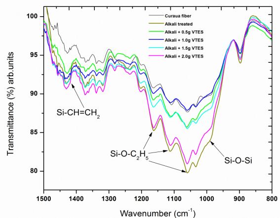
Figure 3. FTIR spectra showing silica peaks of untreated, NaOH treated, and NaOH and silane treated curaua fiber.
